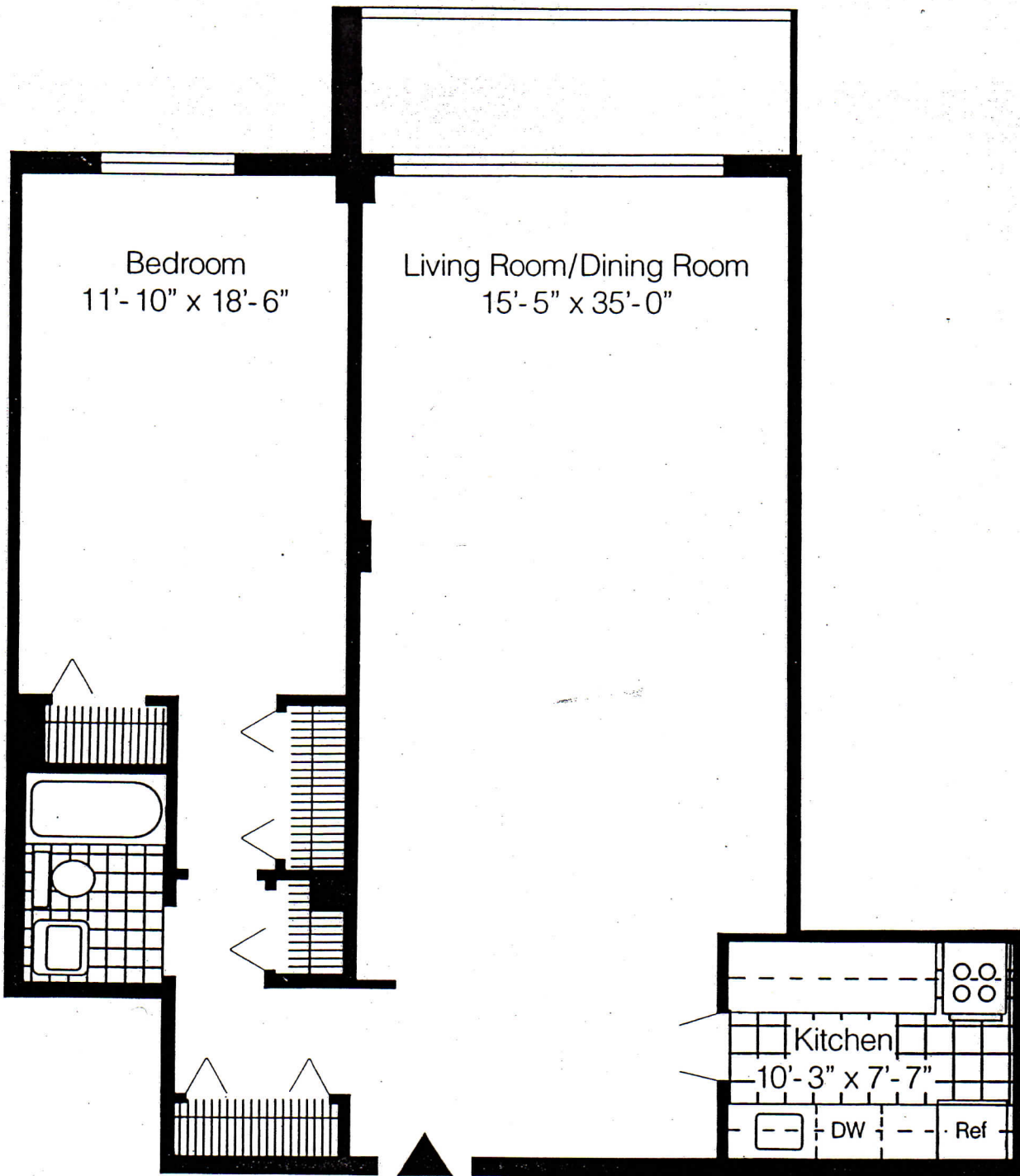
APARTMENT F (Apt. L in reverse) 1 Bedroom/1 Bath 1,046 Sq. Ft.
