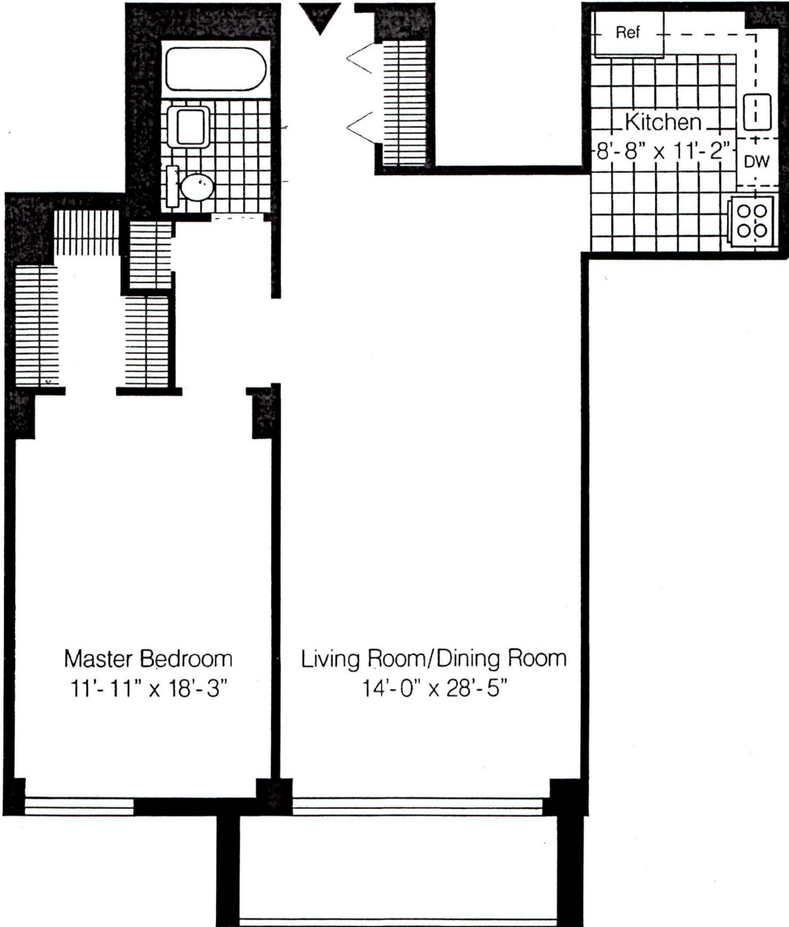
APARTMENT B 1 Bedroom/1 Bath 980 Sq. Ft.
